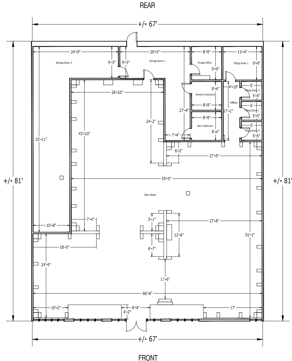
1 MAIN FLOOR
